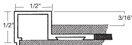
2040 Boxed
