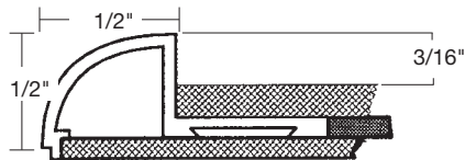
2030 Quarter Round
