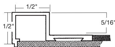
2040 Boxed
