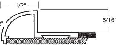
2030 Quarter Round
