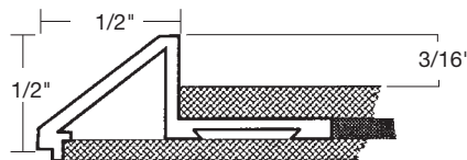
2020 Beveled
